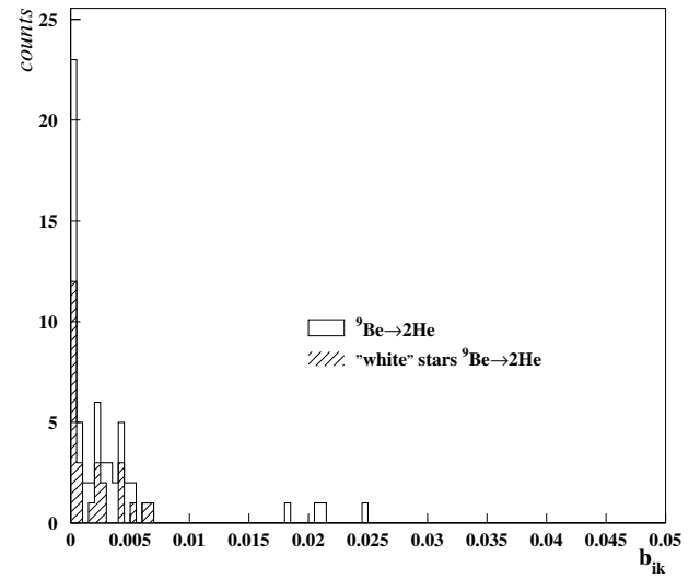
Fig. 6. Distribution of \alpha -particle pairs vs. the relative variable b_{ik} (1) for the fragmentation mode ^9\text{Be} \rightarrow 2\alpha .
