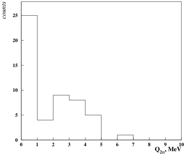
Fig. 7. Distribution of \alpha -particle pairs vs. Q_{2\alpha} (3) for the fragmentation mode {}^9\text{Be} \rightarrow 2\alpha .
