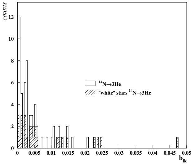
Fig. 4. Distribution of \alpha -particle pairs vs. the relative variable b_{ik} (1) for the fragmentation mode ^{14}\text{N} \rightarrow 3\alpha .
