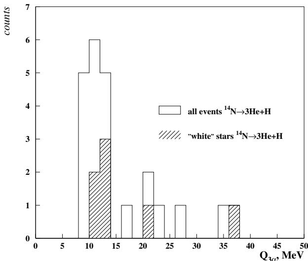
Fig. 5. Distribution of \alpha -particle triplets vs. Q_{3\alpha} (3) for the fragmentation mode ^{14}\text{N} \rightarrow 3\alpha + \text{H} .
