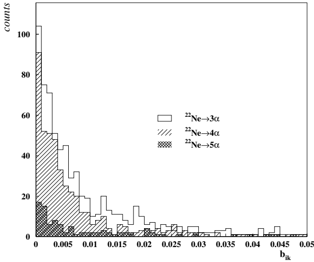
Fig. 2. Distribution of \alpha -particle pairs vs. the relative variable b_{ik} (1) for the fragmentation modes ^{22}\text{Ne} \rightarrow n\alpha .
