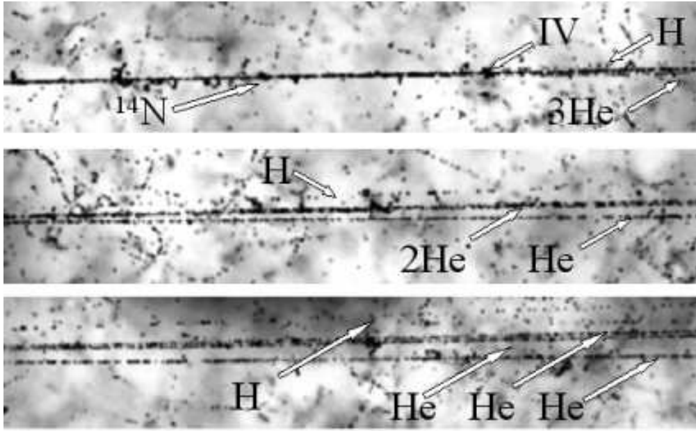
Fig. 1. Example of peripheral interaction of a 2.1 A GeV ^{14}\text{N} nucleus in a nuclear track emulsion (“white” star). The interaction vertex (indicated as IV) and nuclear fragment tracks (H and He) in a narrow angular cone are seen on the upper microphotograph. Following the direction of the fragment jet, it is possible to distinguish 1 singly and 3 doubly charged fragments on the middle and bottom microphotograph.
